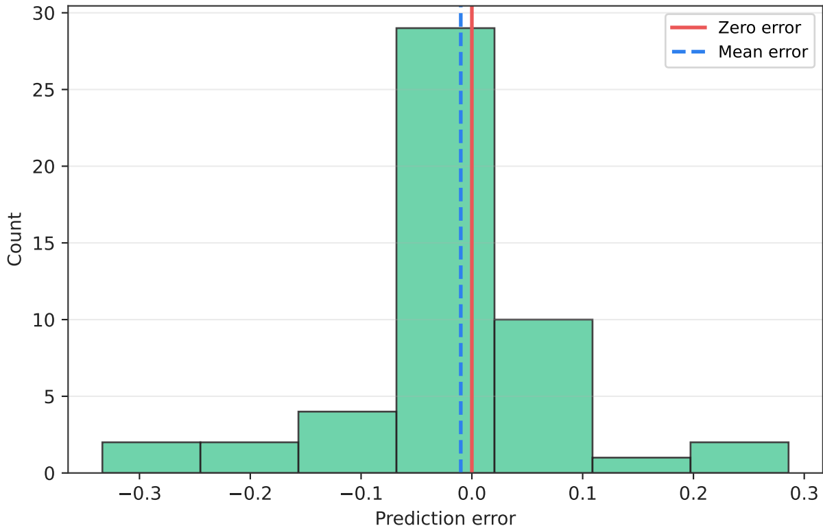
Residual Distribution: pH adjustment
